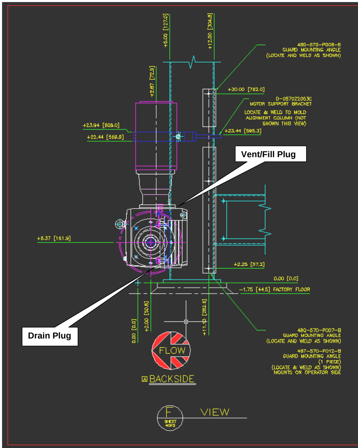
Locations of fill and drain plugs for bender conveyor helical worm gearbox
